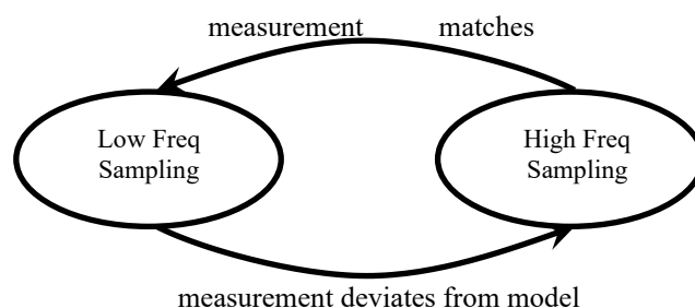
Figure 3: Basic time-division scheduler
